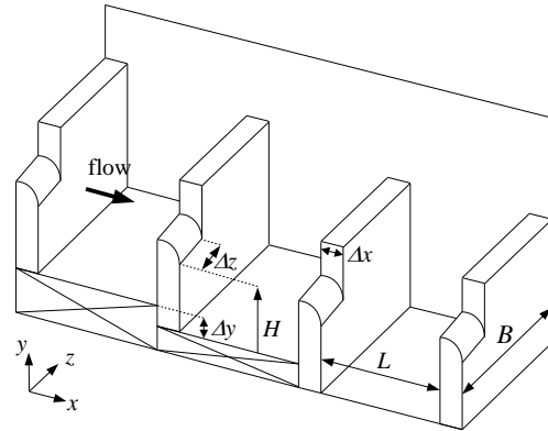
Figure 1, Pool-and-weir fishway
